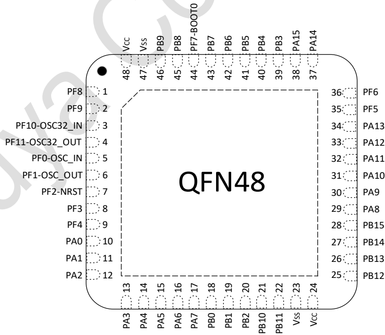
图 3-2 QFN48 Pinout1 PY32F031C1xU (Top view)
