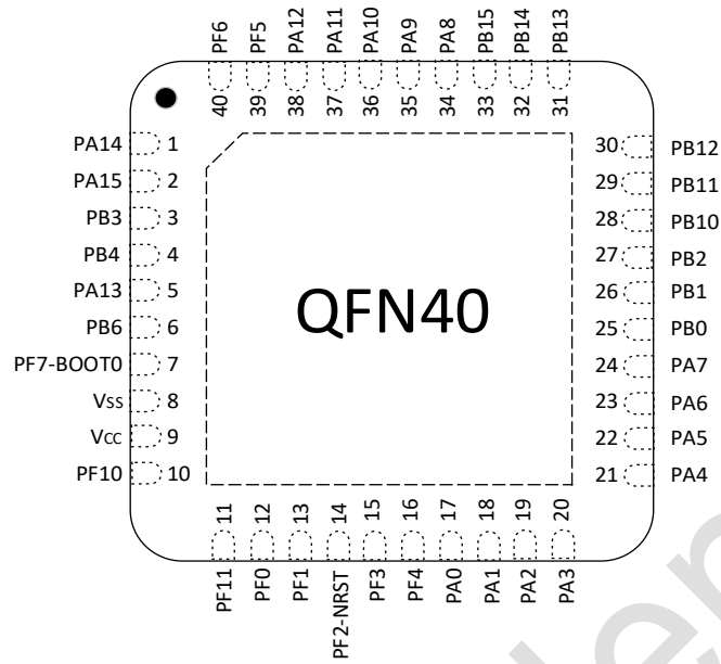
图 3-3 QFN40 Pinout1 PY32F031H1xU (Top view)
