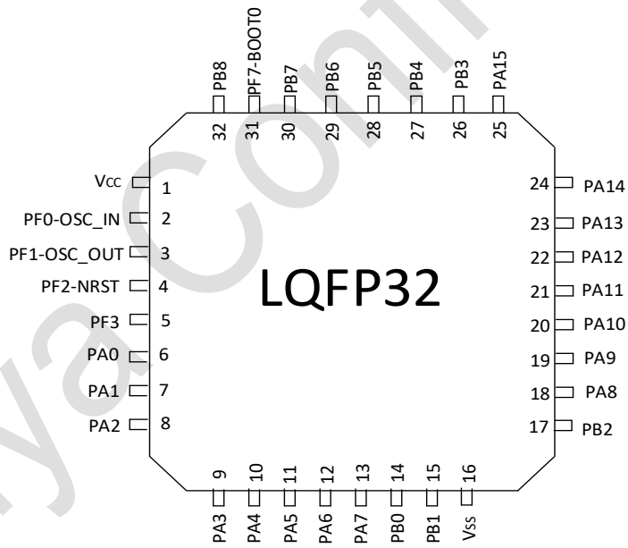
图 3-4 LQFP32 Pinout1 PY32F031K1xT (Top view)
