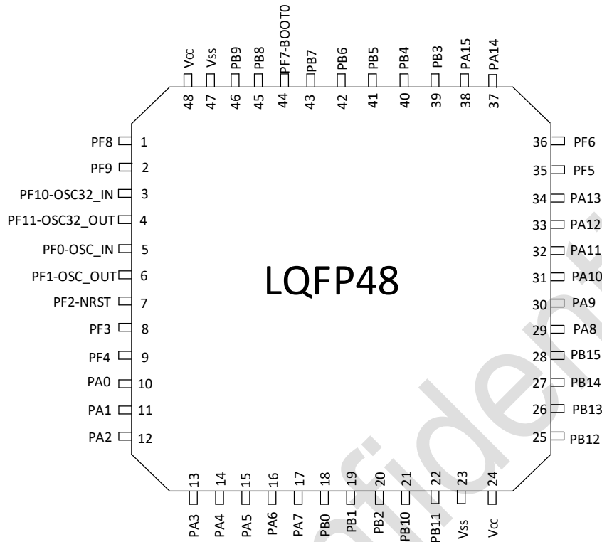
图 3-1 LQFP48 Pinout1 PY32F031C1xT (Top view)
