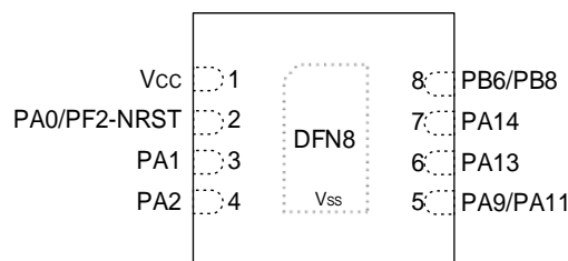
图 3-7 DFN8(2*2) Pinout1 PY32F031L1xD (Top view)
